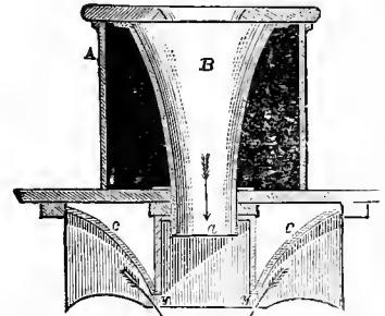
Fig. 3842. Enlarged Section.
